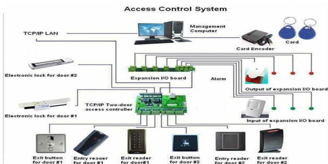
Figure 1 Access Control System Architecture
